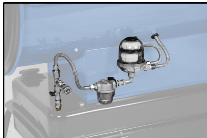
DEAERATOR KIT (TIGERLOOP)
