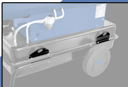
(4) LIFTING BRACKETS
